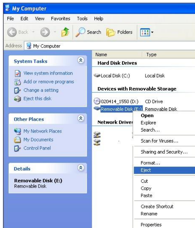
Figure 65 - My Computer/Eject
