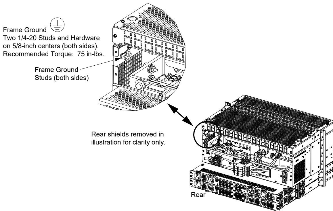
Figure 1 System Shelf Frame Grounding Connection
