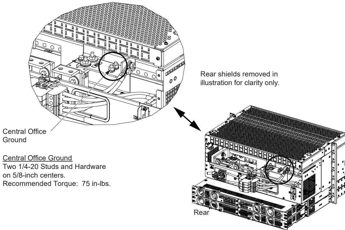
Figure 2 Central Office Ground Connection
