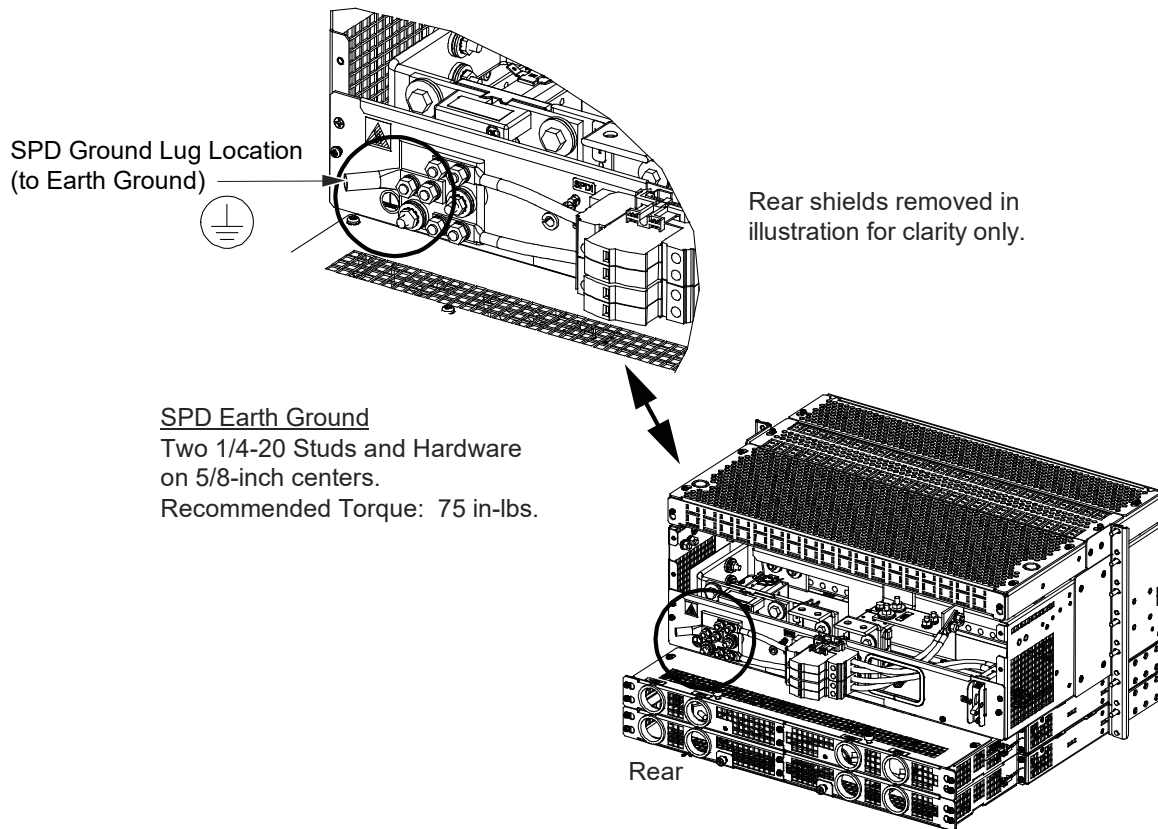
Figure 3 SPD (Surge Protection Device) Earth Ground Connection
