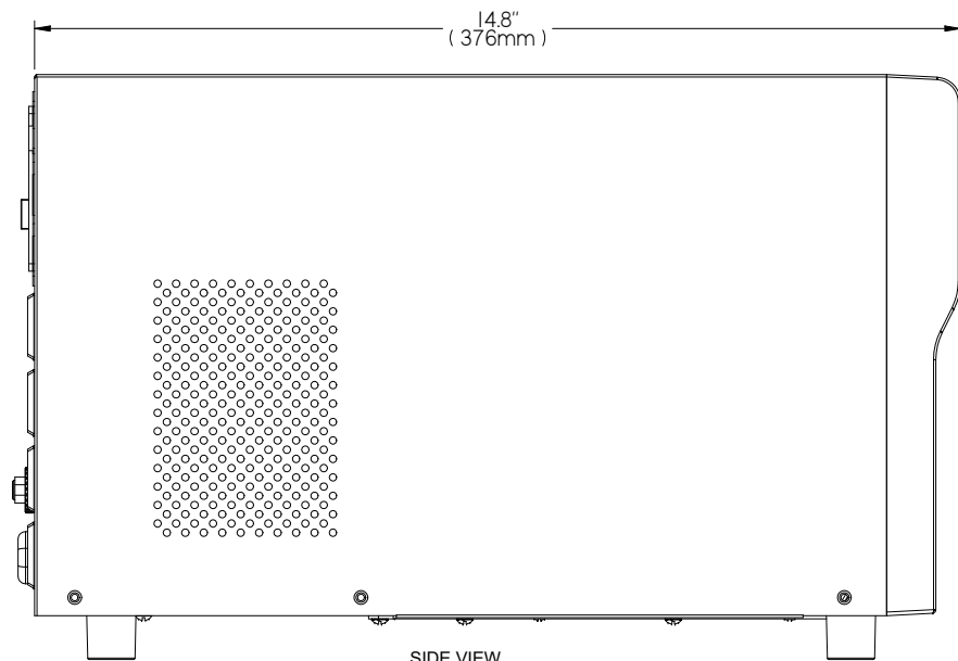
SIDE VIEW
