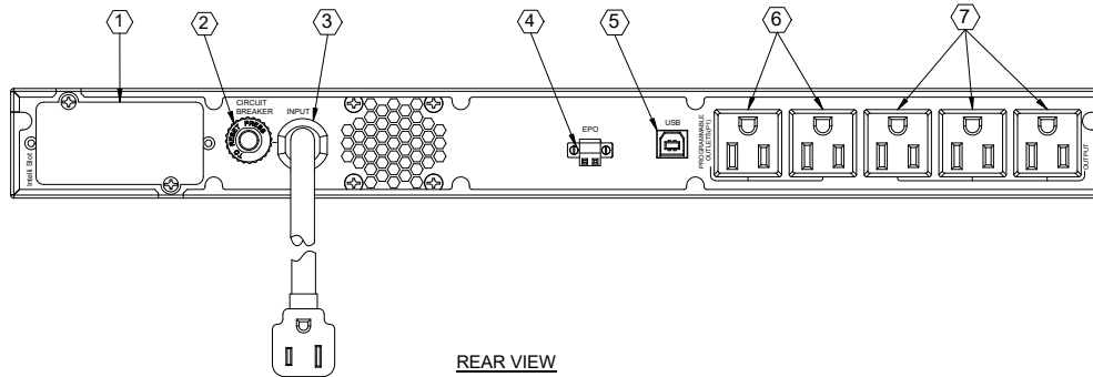
REAR VIEW
