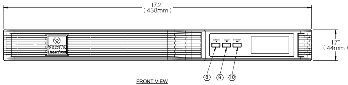
FRONT VIEW
