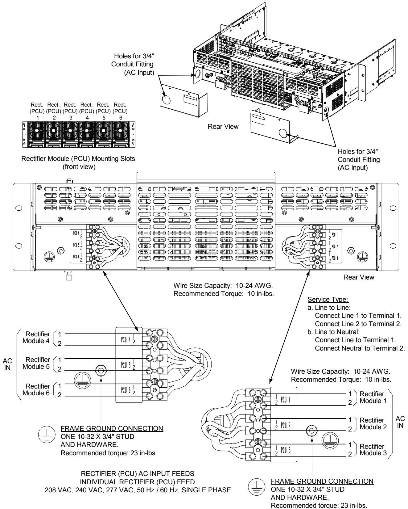
Figure 1 List 1 and 31 AC Input and Frame Ground Connections (Single-Phase Input) (Terminal Blocks)
