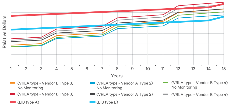
Figure 4: Models VRLA and LIB over 15 year at 5 minutes of runtime
