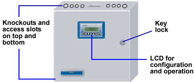
Liebert AC8 enclosure - External features
