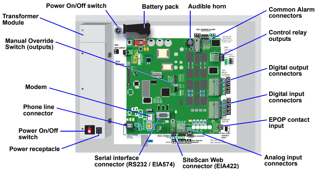
Liebert AC8 Components and Key Features
